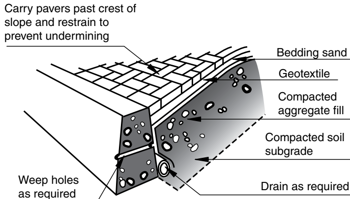
Figure 6. Embankment with concrete pavers
