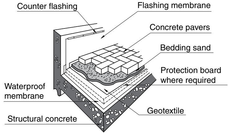
Figure 3. Roof assembly
