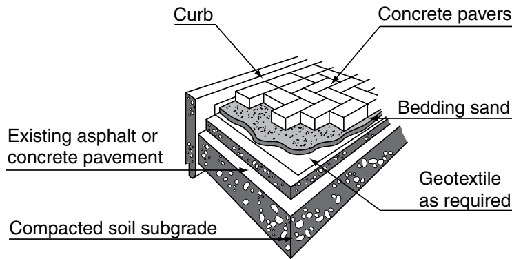
Figure 5. Typical overlay/inlay on existing pavement.
