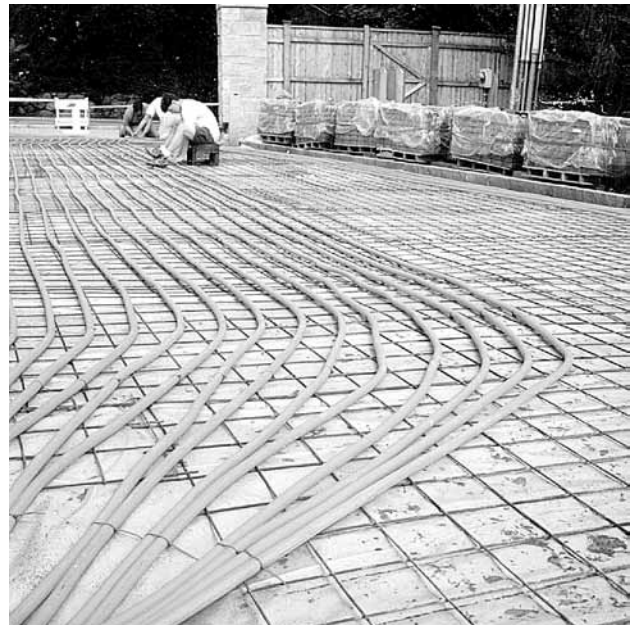
Figure 4. The heating system is tied to a wire mesh anchored into the compacted aggregate base.
