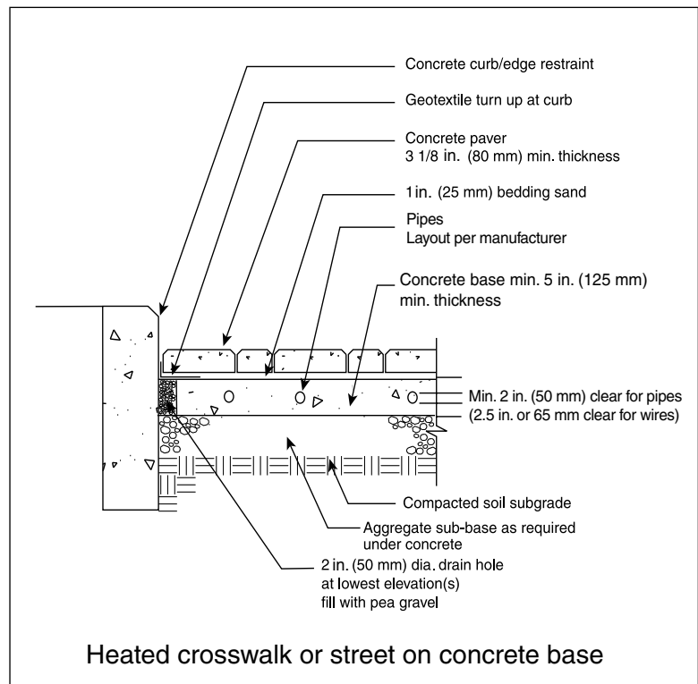
Figure 5. A typical cross section of a heated interlocking concrete pavement for crosswalks and roads subject to vehicular traffic. For asphalt bases, pipes should be located at least 1\frac{1}{2} in. (40 mm) under the asphalt.
