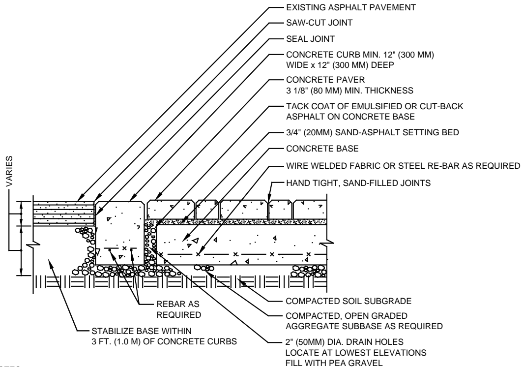
Figure 7. Crosswalk with an asphalt base
